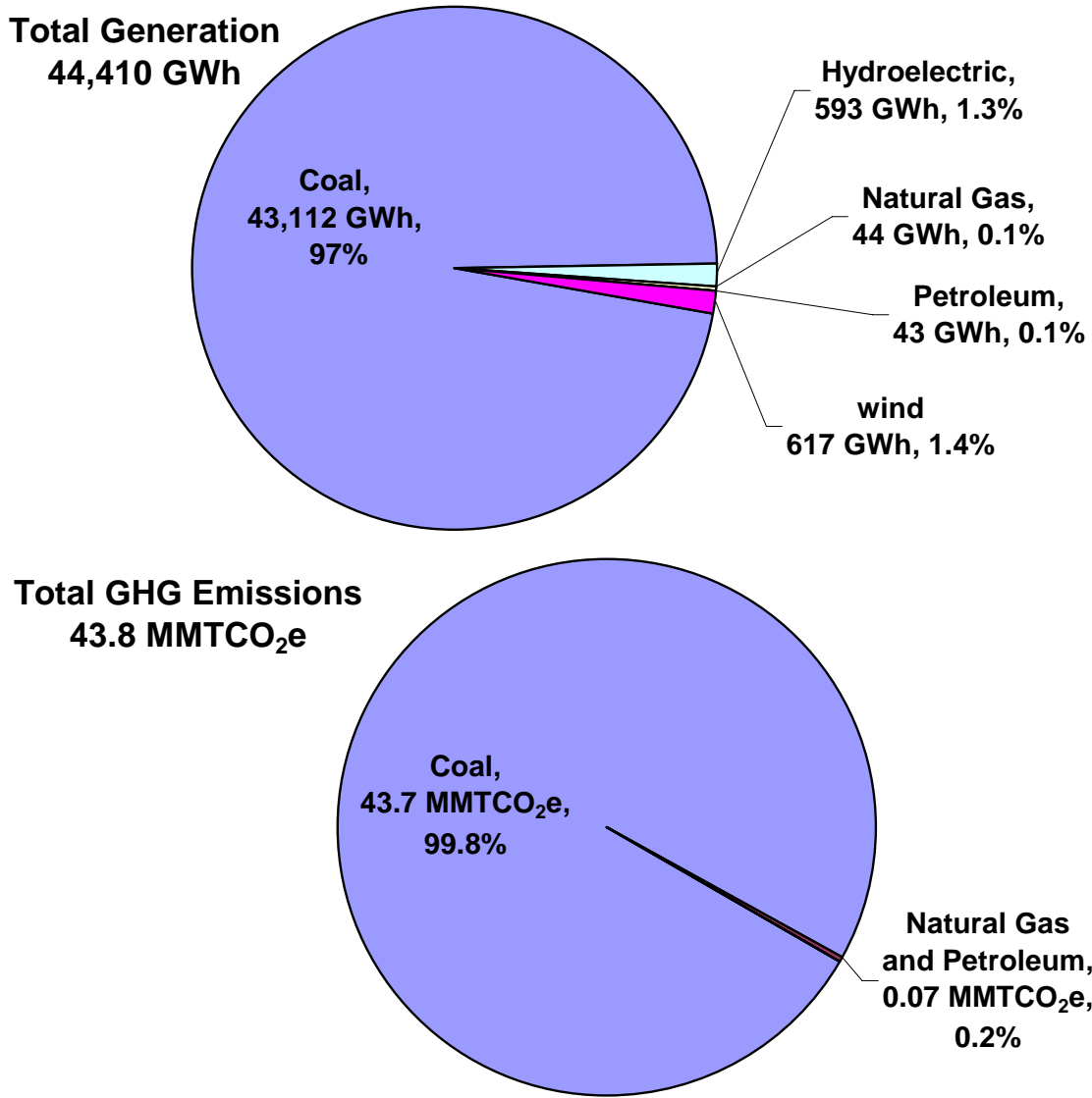
Figure A3. Electricity Generation and GHG Emissions from Wyoming Power Plants, 2004
