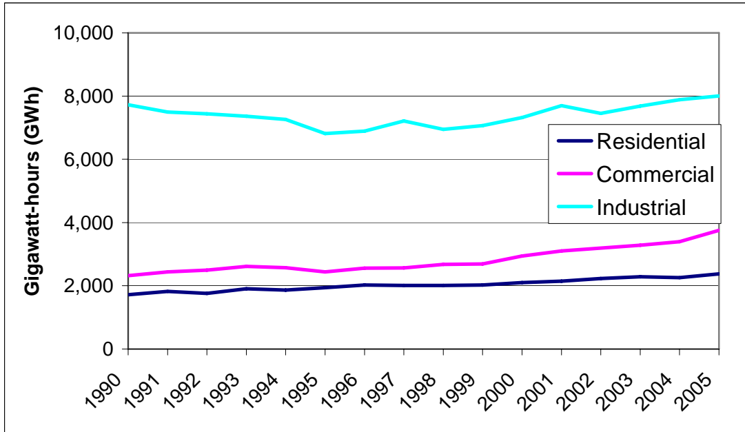
Figure A2. Electricity Consumption by Sector in Wyoming, 1990-2005 17
