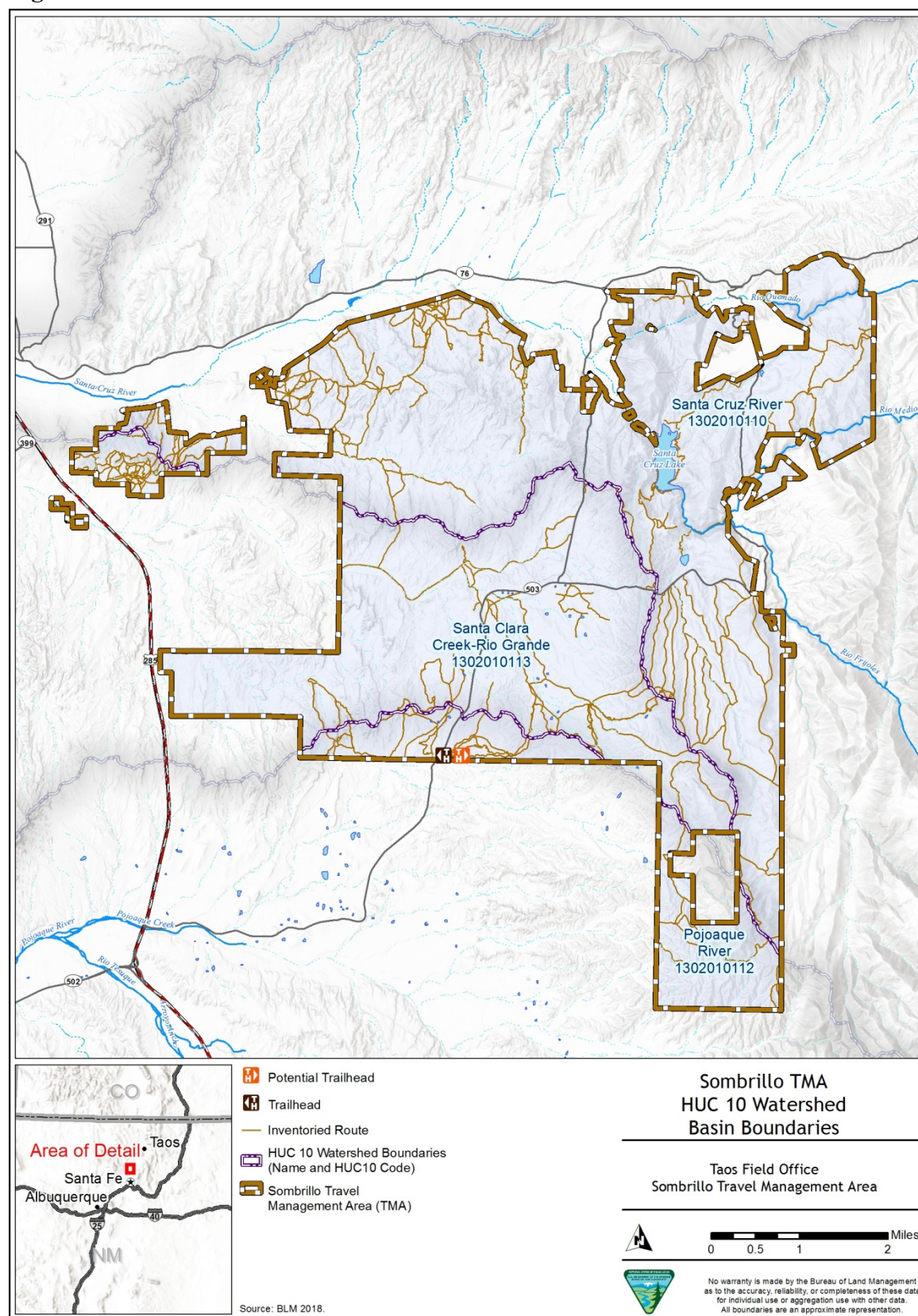
Figure 3.5-1. Watershed Basin Boundaries
