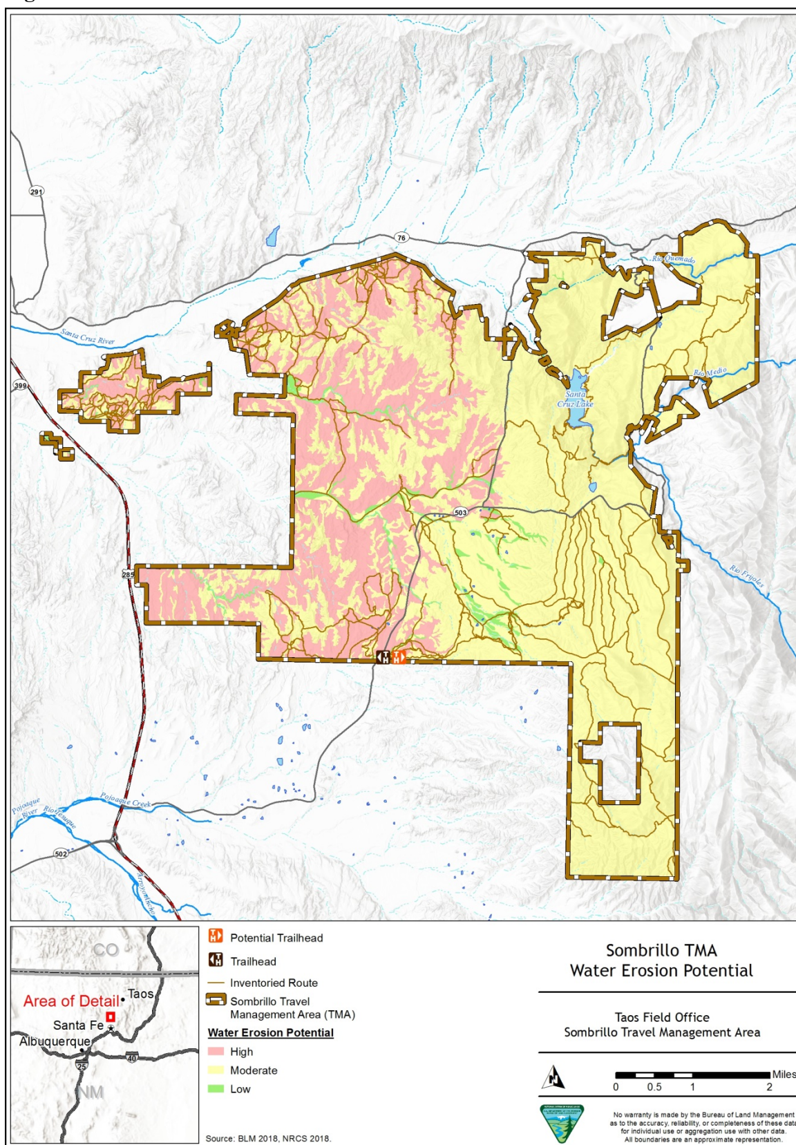
Figure 3.5-2. Water Erosion Potential
