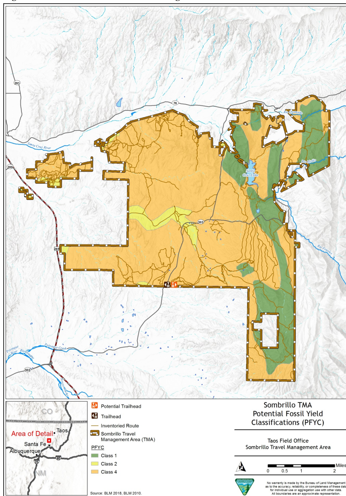
Figure 3.4-1. PFYC Classes for Paleontological Resources
