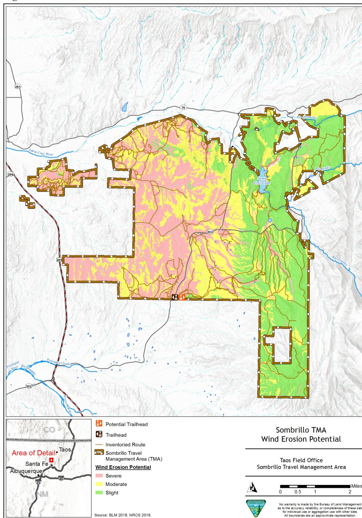
Figure 3.5-3. Wind Erosion Potential
