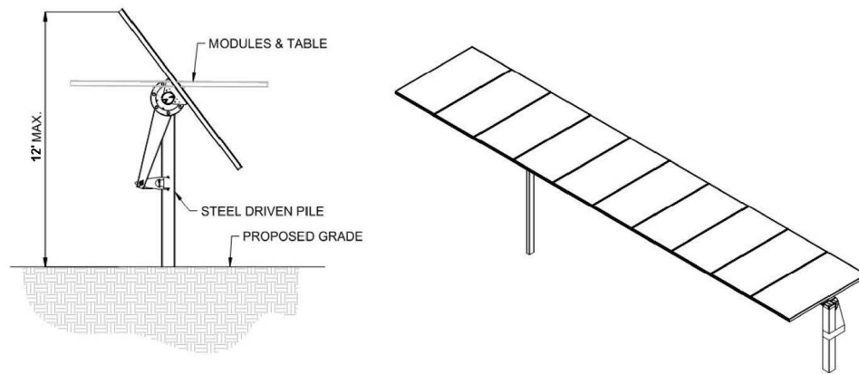
SINGLE AXIS TRACKER NOT TO SCALE
