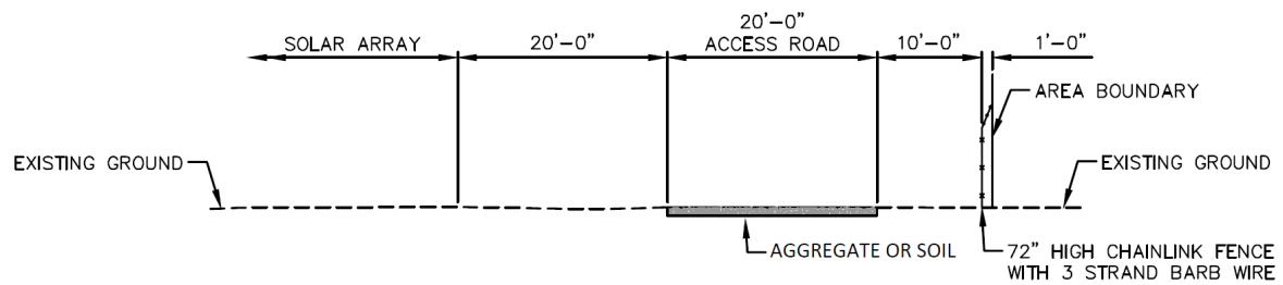
FIGURE 1-7 CROSS SECTION OF A TYPICAL ROAD
