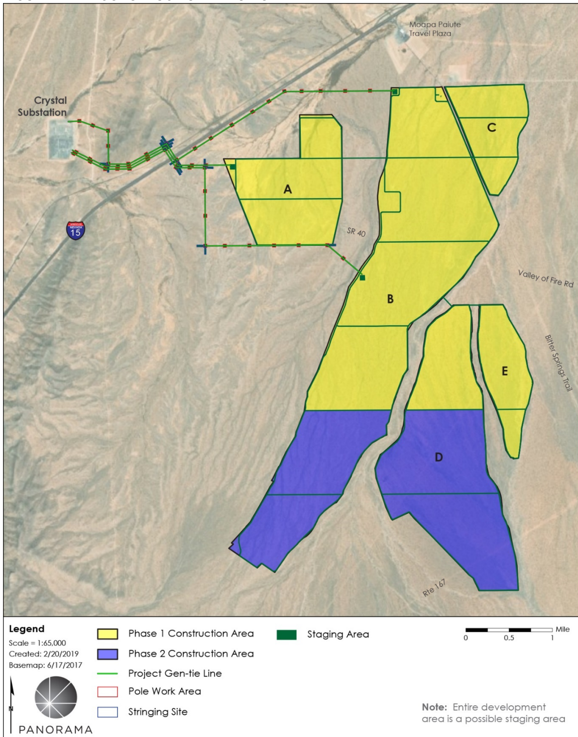
FIGURE 2-1 CONSTRUCTION PHASING
