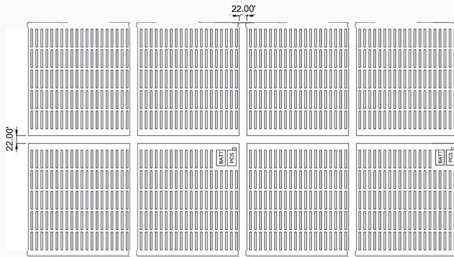
TYPICAL TRACKER ARRAY BLOCKS WITH PCS AND BATTERY
