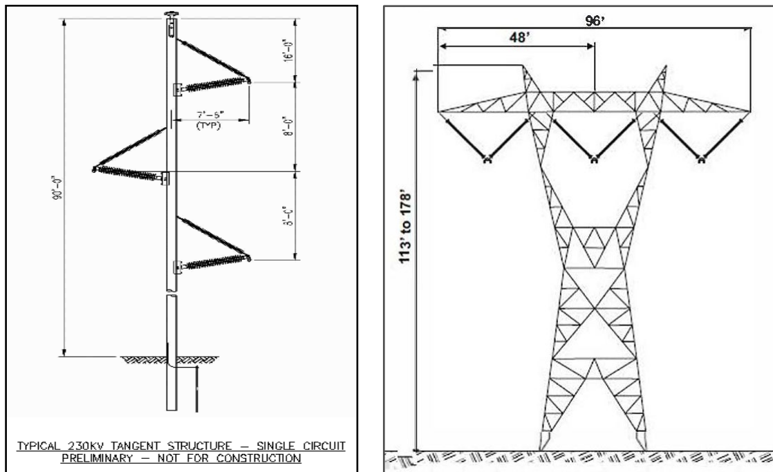
FIGURE 1-14 TYPICAL GEN-TIE SUPPORT STRUCTURES FOR 230 KV AND 500 KV LINES
