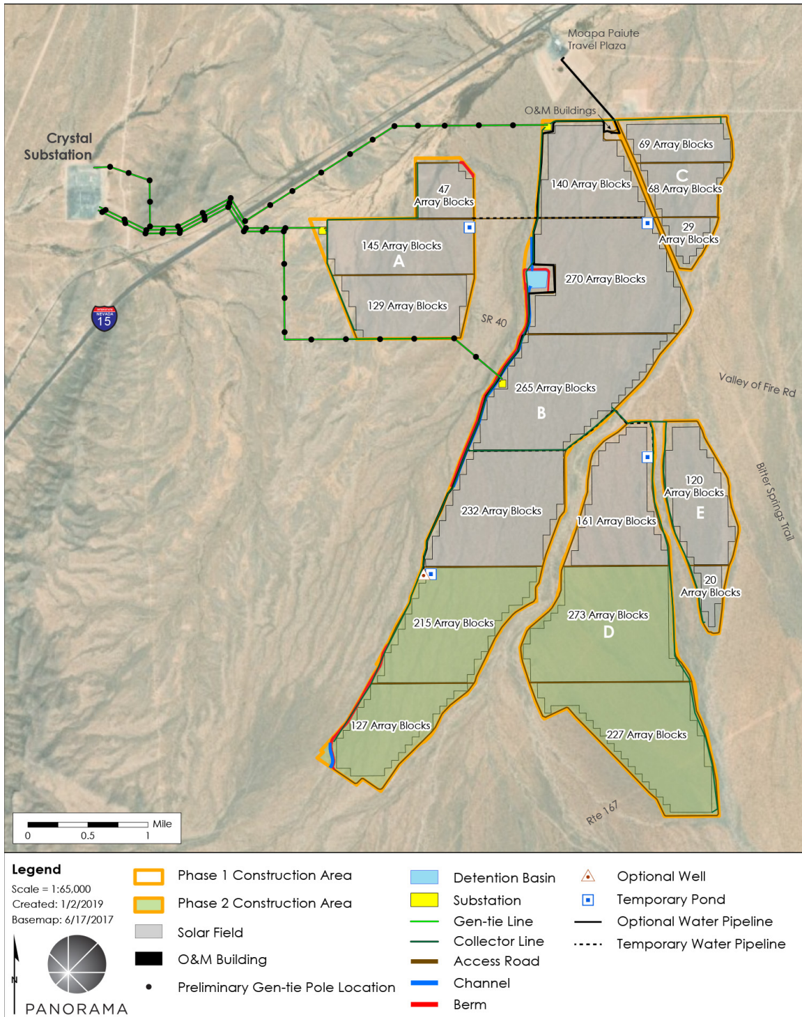
FIGURE 1-2 PROJECT ELEMENTS
