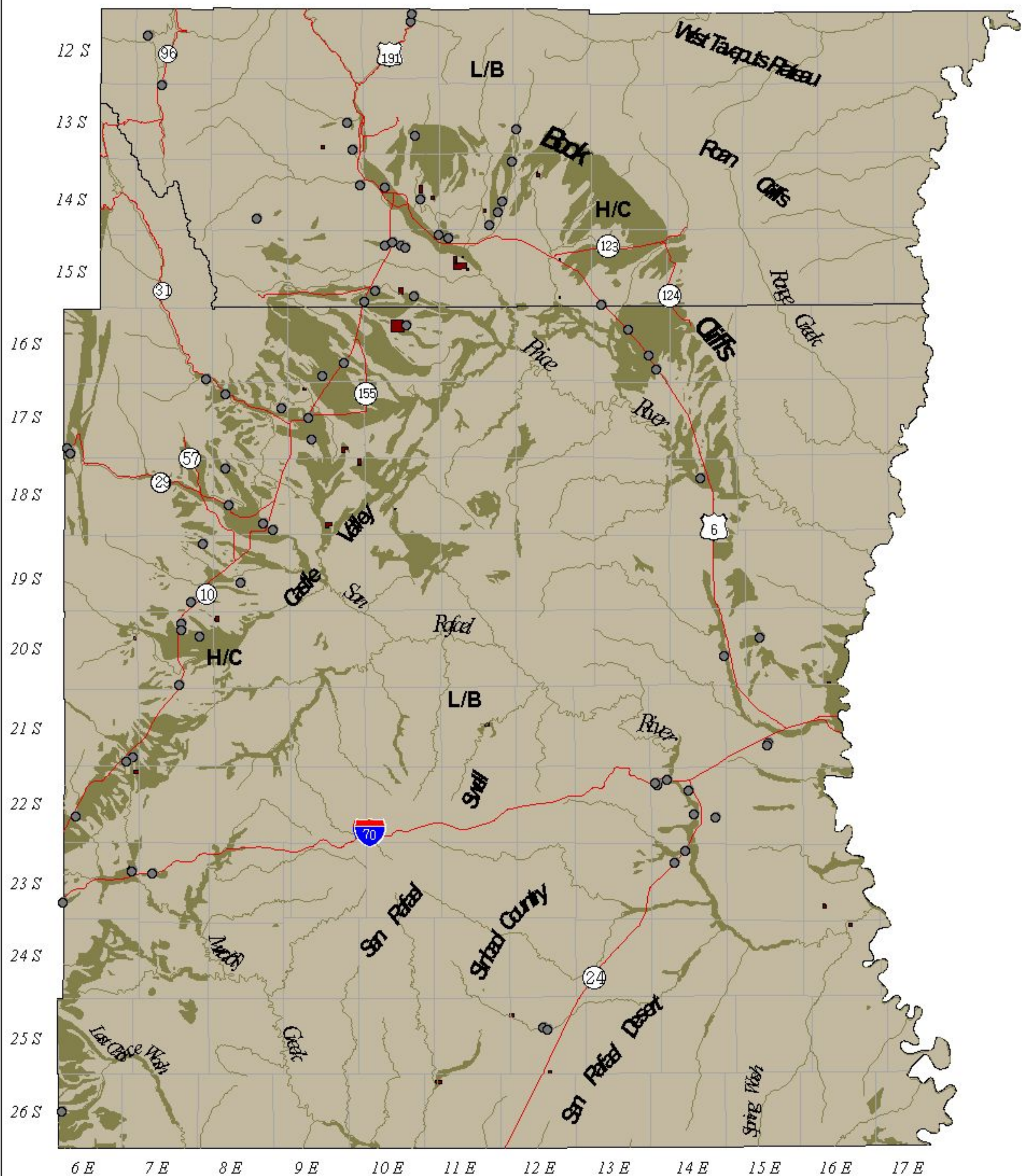
Map 36: Sand and Gravel Occurrence Potential in the Planning Area
