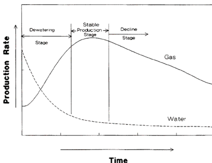
Figure 3-6. CBNG Well Production Profile
