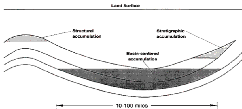
Figure 3-2. Petroleum Traps
