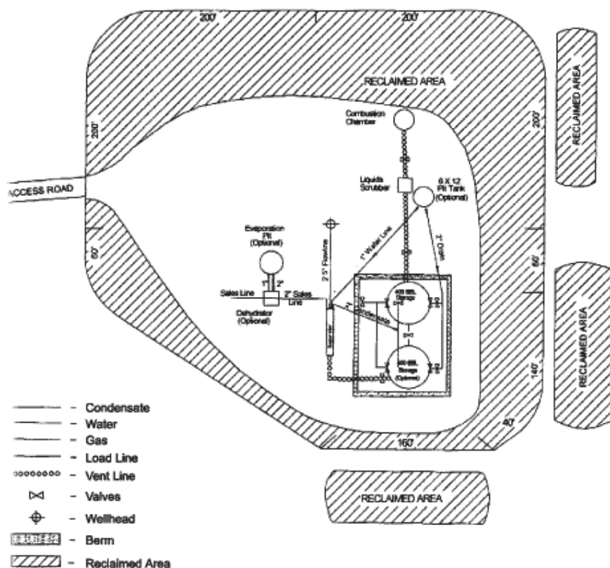
Figure 5. Typical Gas Well Production Facility
