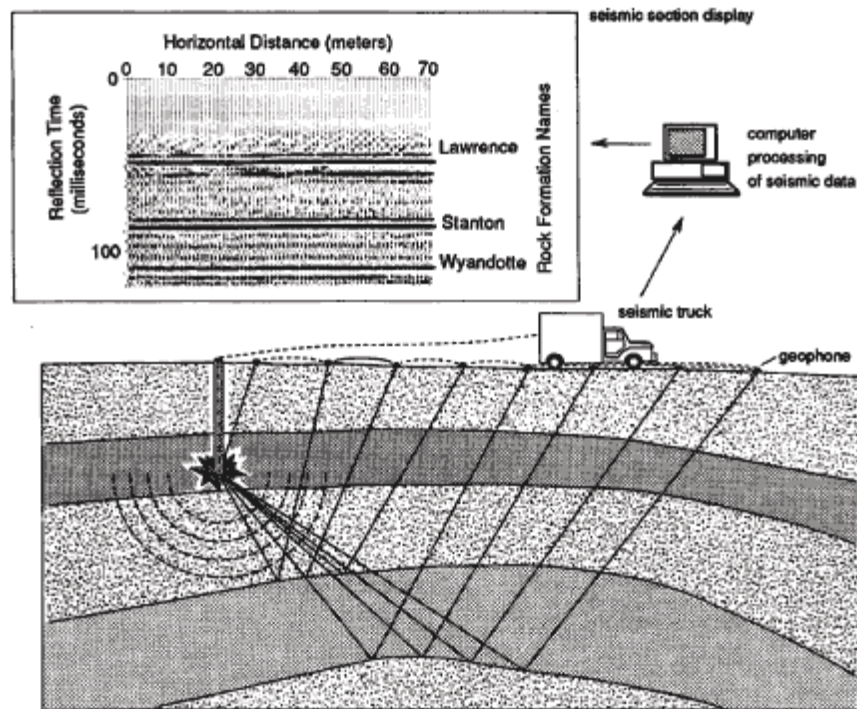
Figure 1. Seismic Survey Process
