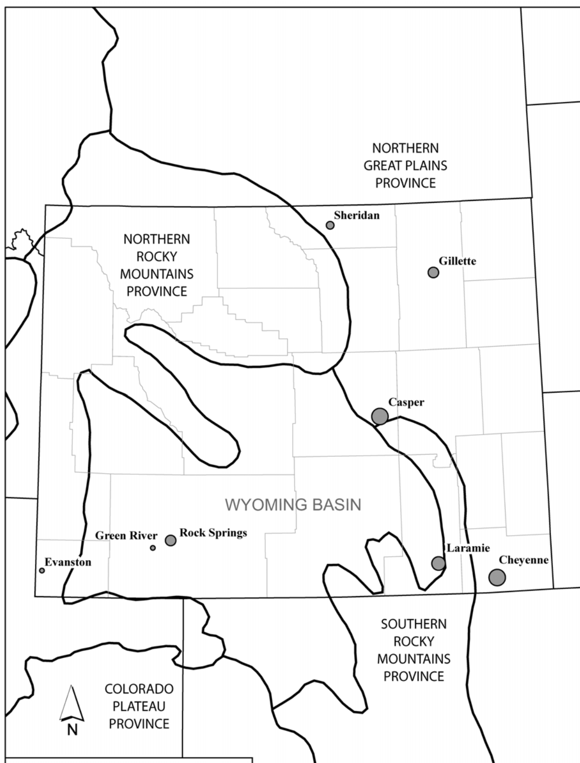
Figure 2-1. Wyoming Physiographic Provinces
