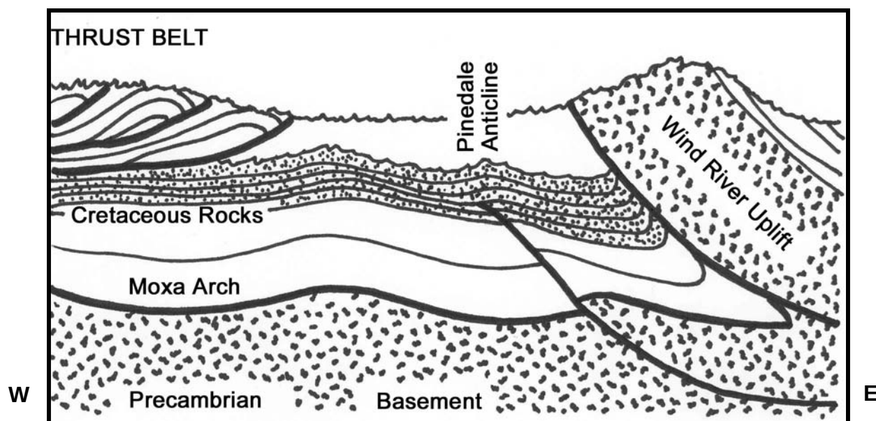
Figure 2-5. Green River Basin Cross-Section
