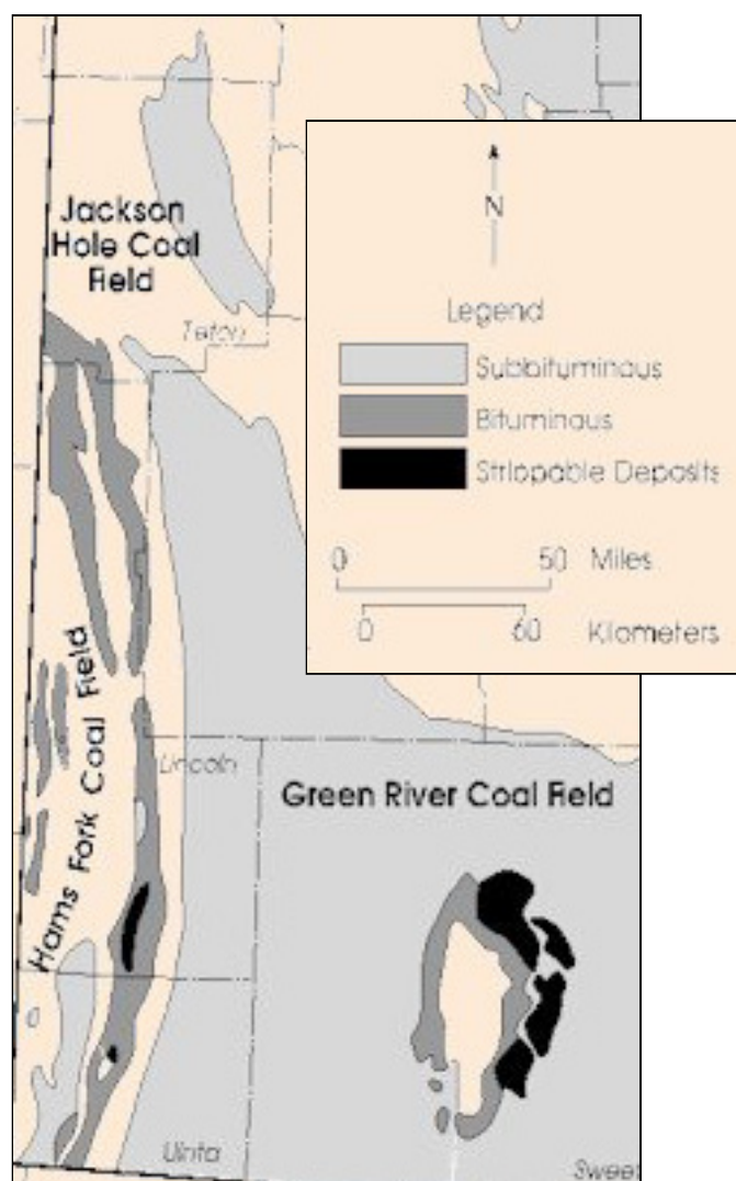
Figure 3-8. Kemmerer Planning Area Regional Coal Fields
