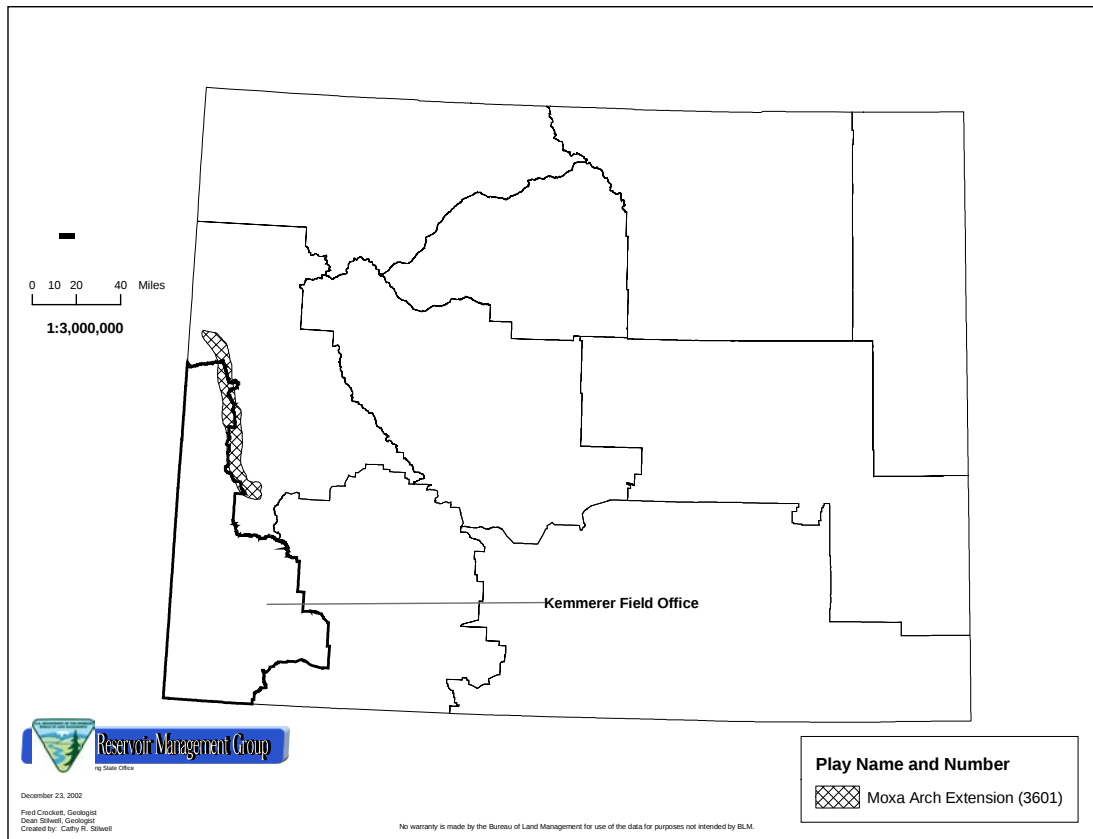
Figure 4-1. Moxa Arch Extension Play
