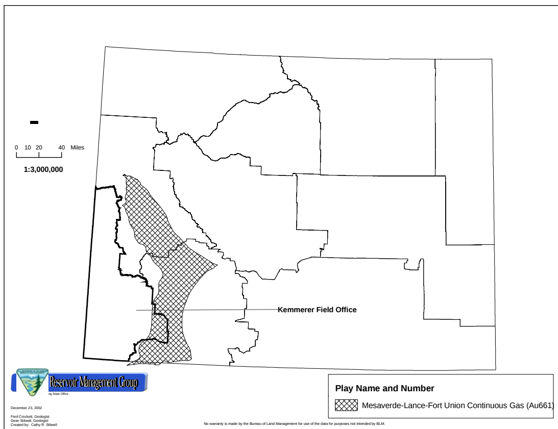
Figure 4-7. Mesaverde-Lance-Fort Union Continuous Gas Play
