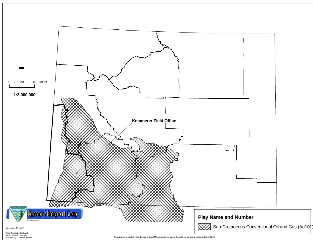
Figure 4-12. Sub-Cretaceous Conventional Oil and Gas Play
