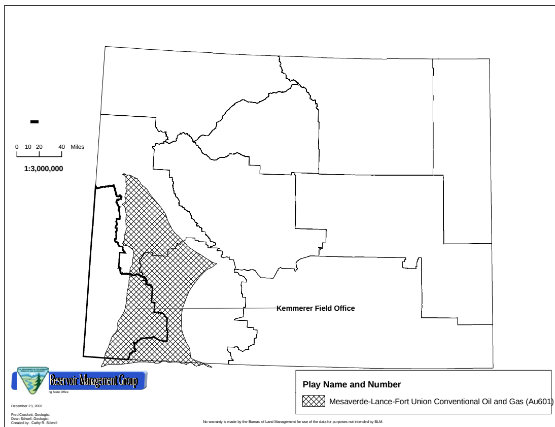
Figure 4-8. Mesaverde-Lance-Fort Union Conventional Oil and Gas Play
