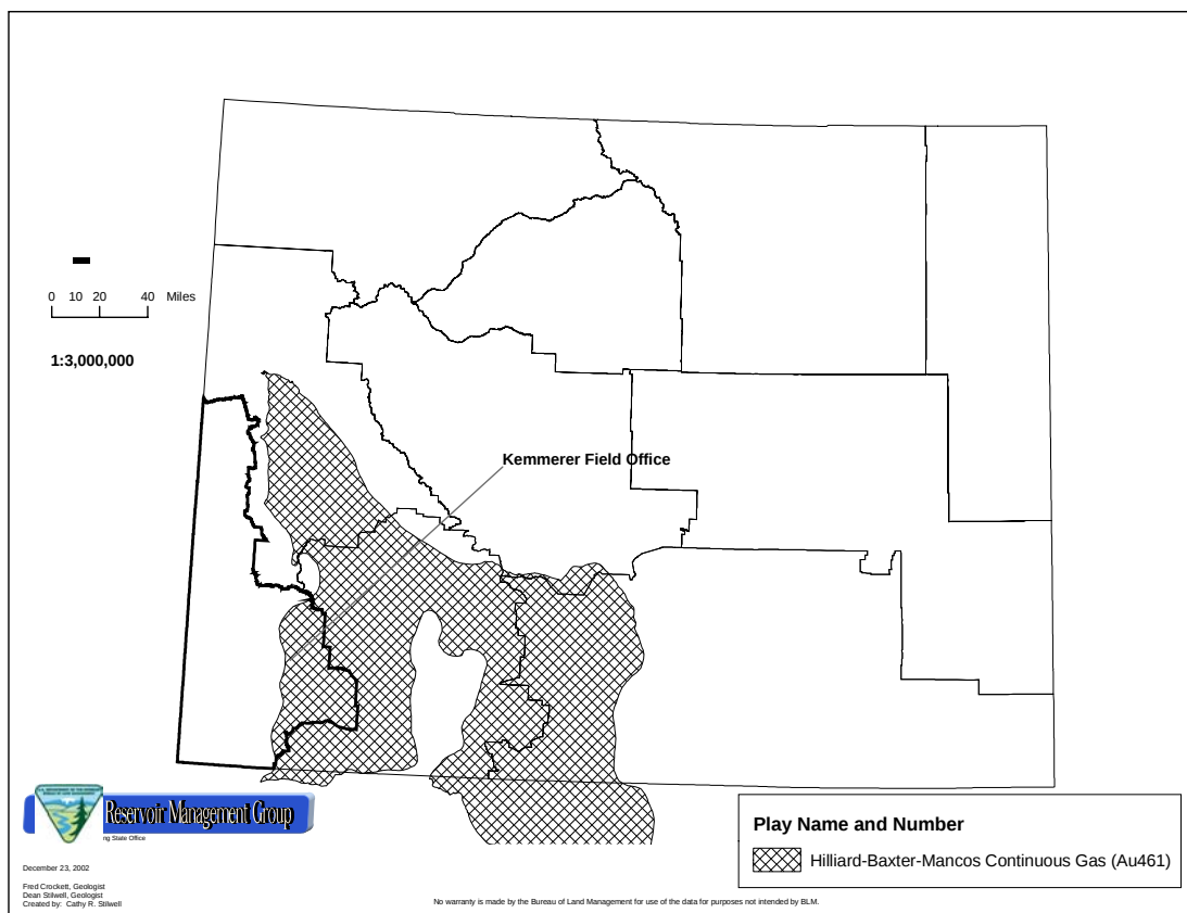
Figure 4-9. Hilliard-Baxter-Mancos Continuous Gas Play
