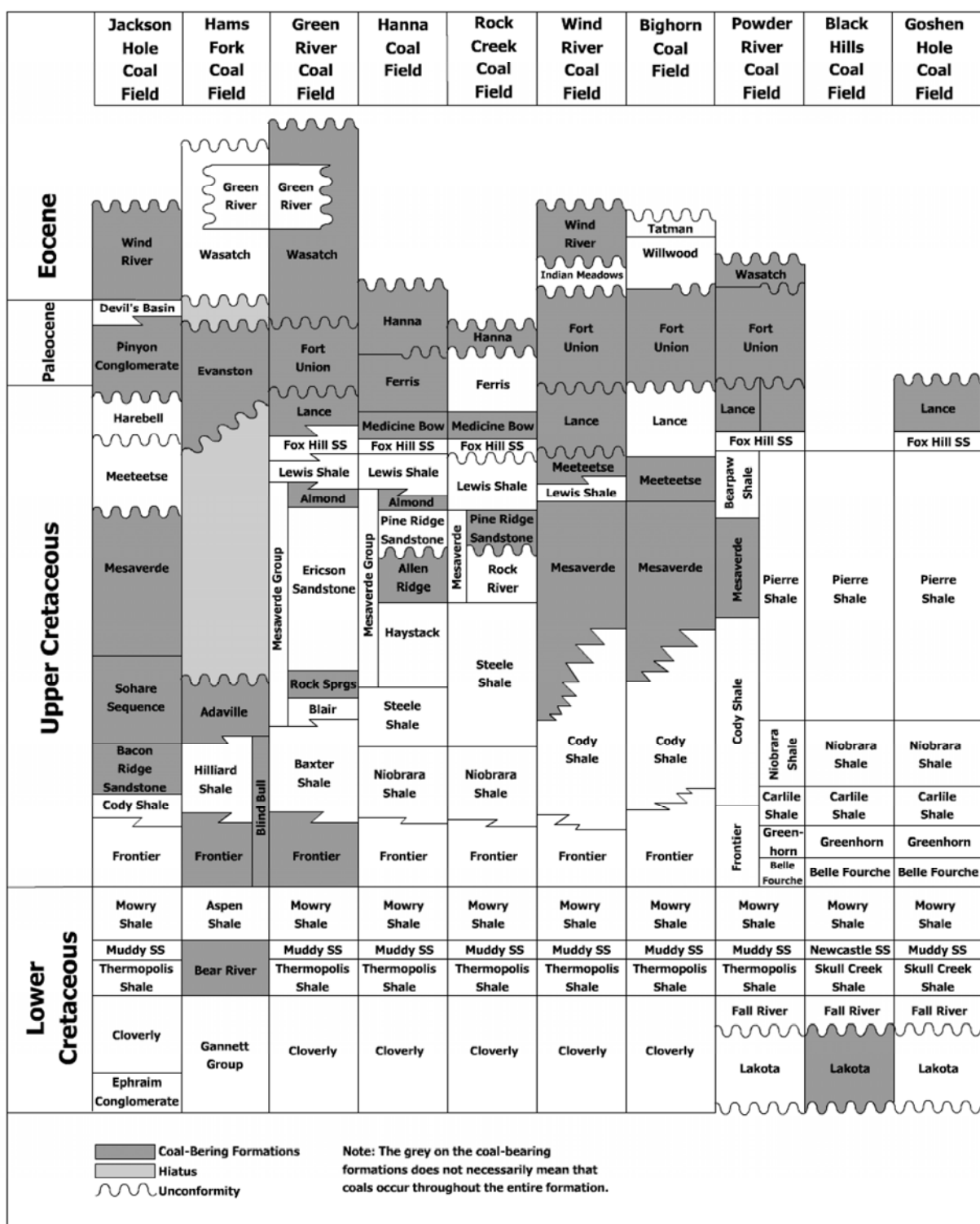
Figure 3-7. Wyoming Coal-Bearing Formations
