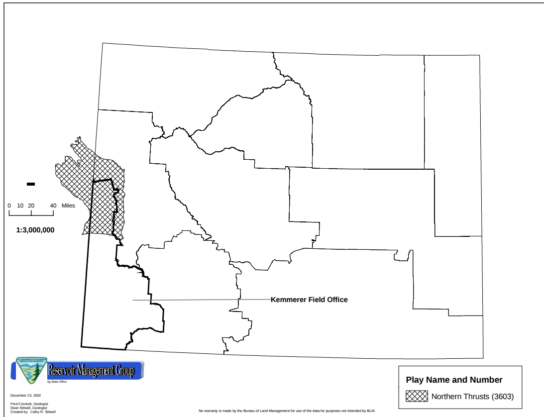
Figure 4-3. Northern Thrusts Play
