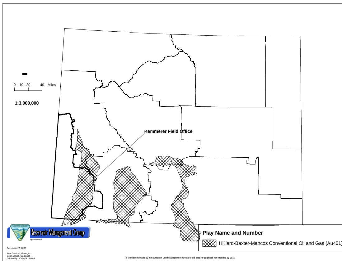
Figure 4-10. Hilliard-Baxter-Mancos Conventional Oil and Gas Play
