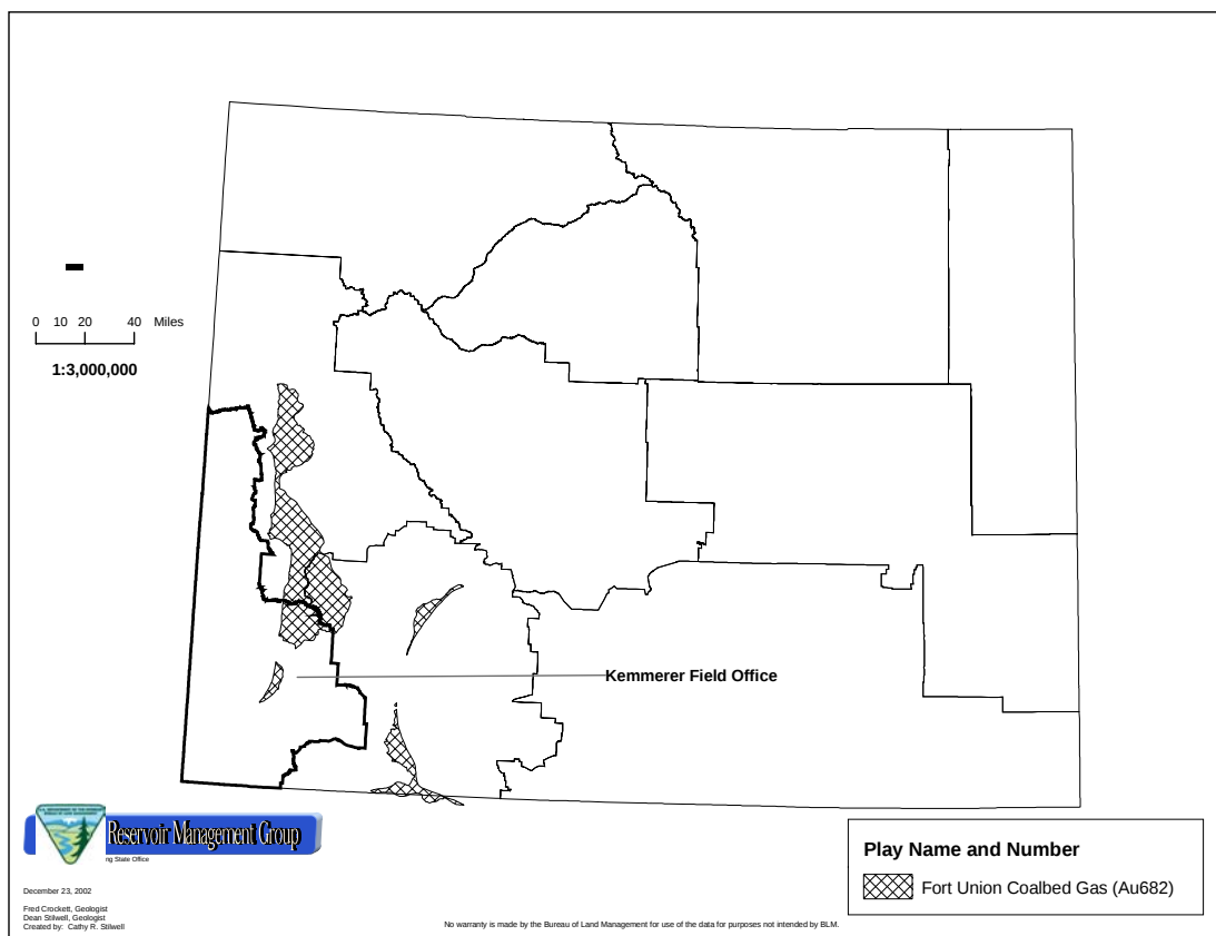
Figure 4-19. Fort Union Coalbed Gas Play
