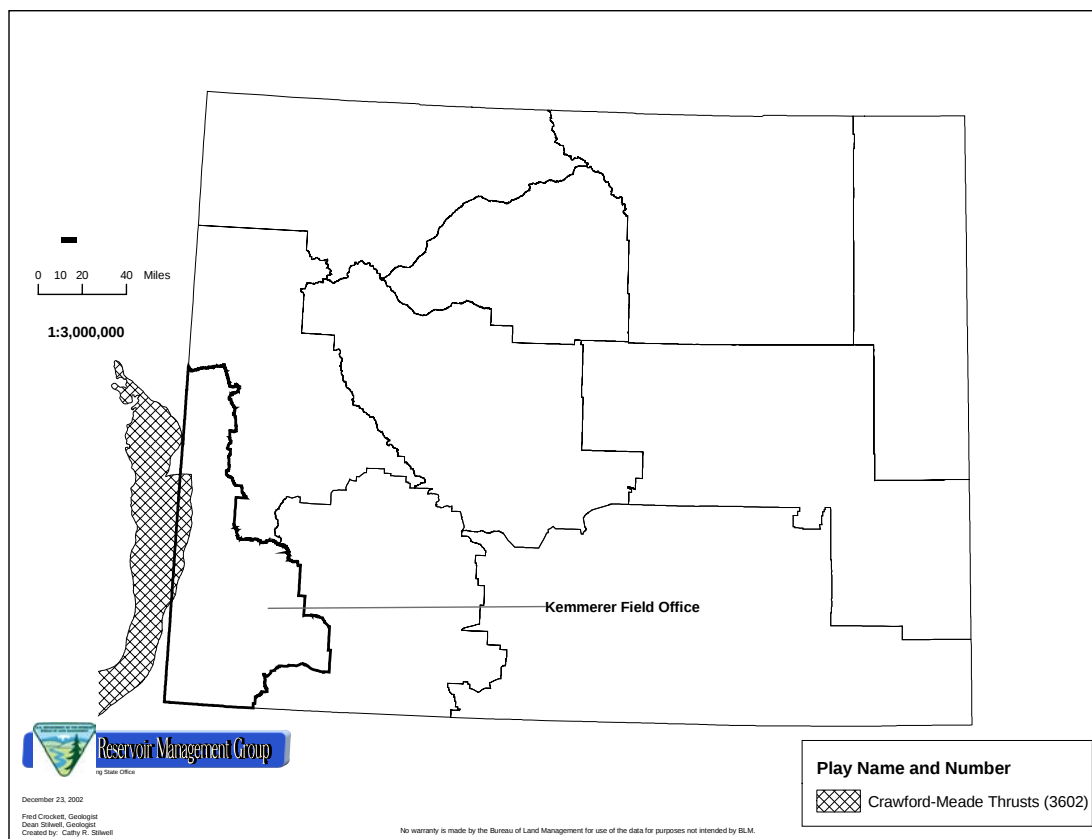
Figure 4-2. Crawford-Meade Thrusts Play
