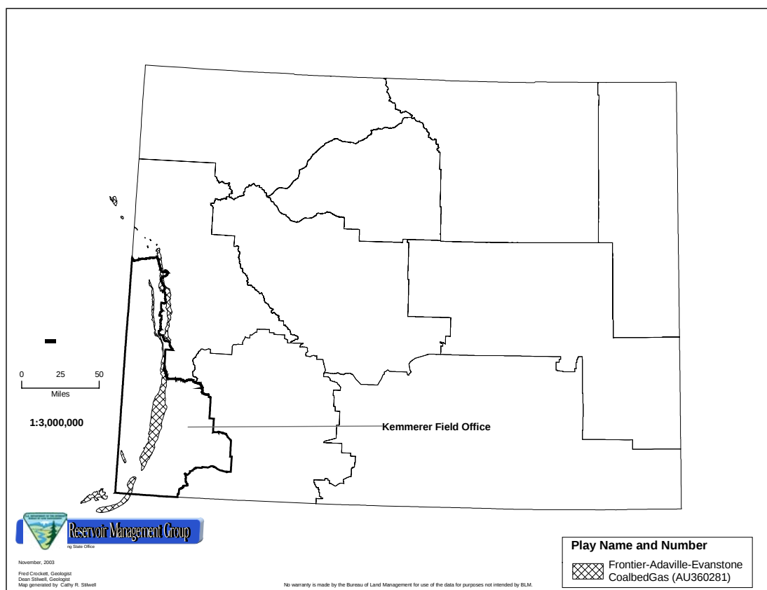
Figure 4-18. Frontier-Adaville-Evanston Coalbed Gas Play
