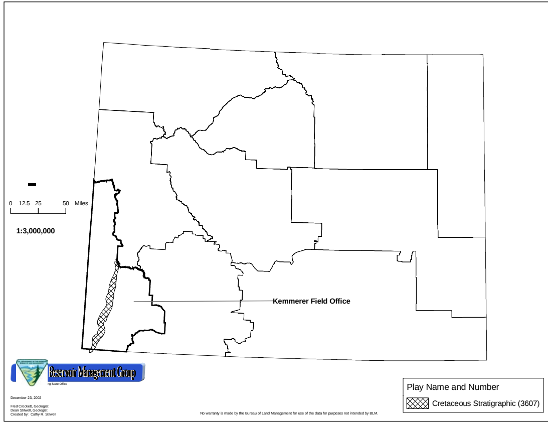
Figure 4-5. Cretaceous Stratigraphic Play
