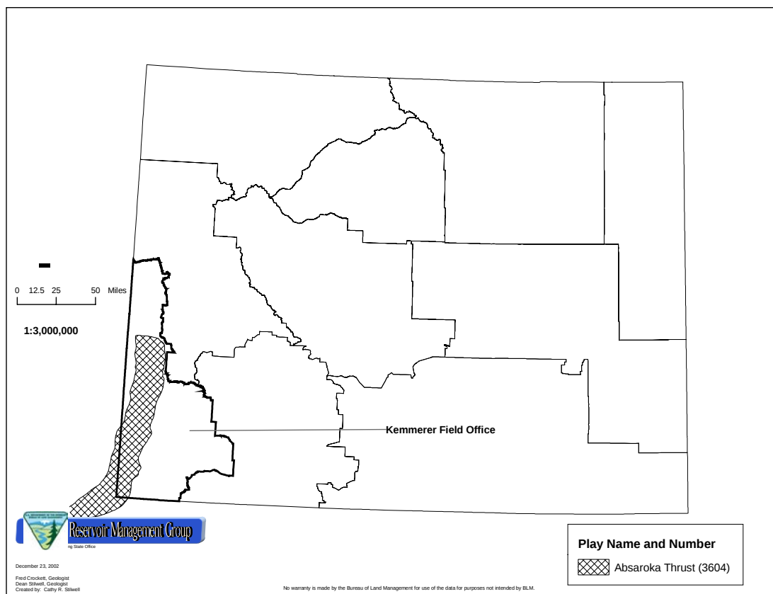
Figure 4-4. Absaroka Thrust Play
