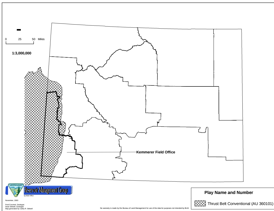
Figure 4-11. Thrust Belt Conventional Play
