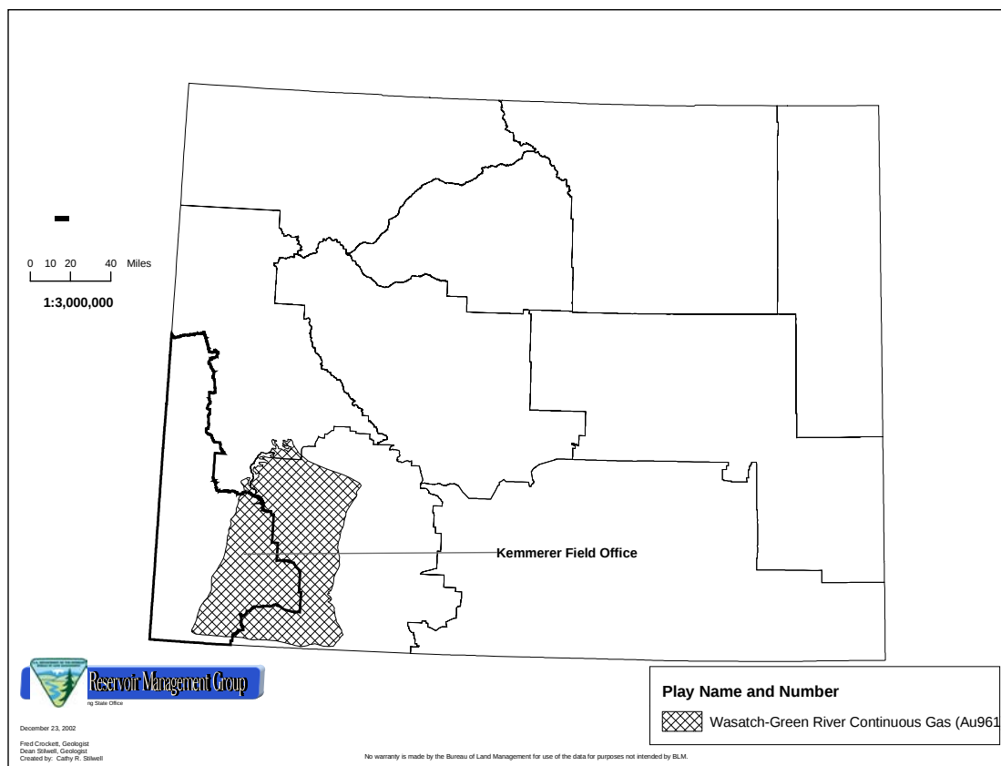
Figure 4-6. Wasatch-Green River Continuous Gas Play
