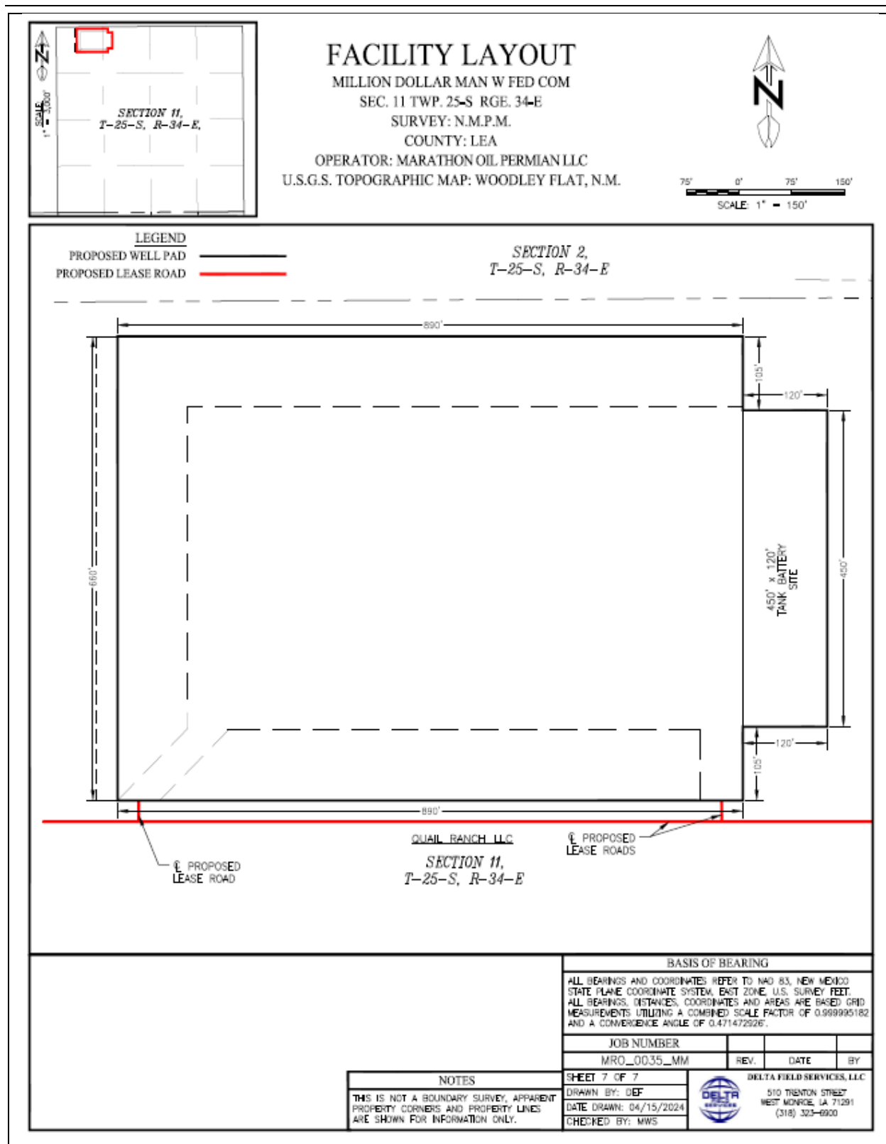
Figure 2.5. Location of Proposed Central Tank Battery
