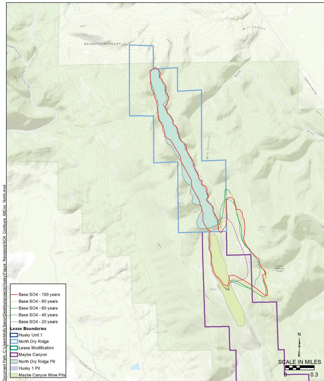
Figure 31. Predicted Sulfate Plumes at 20-year Intervals, Alternative Cover from NDR and North Maybe Mine
