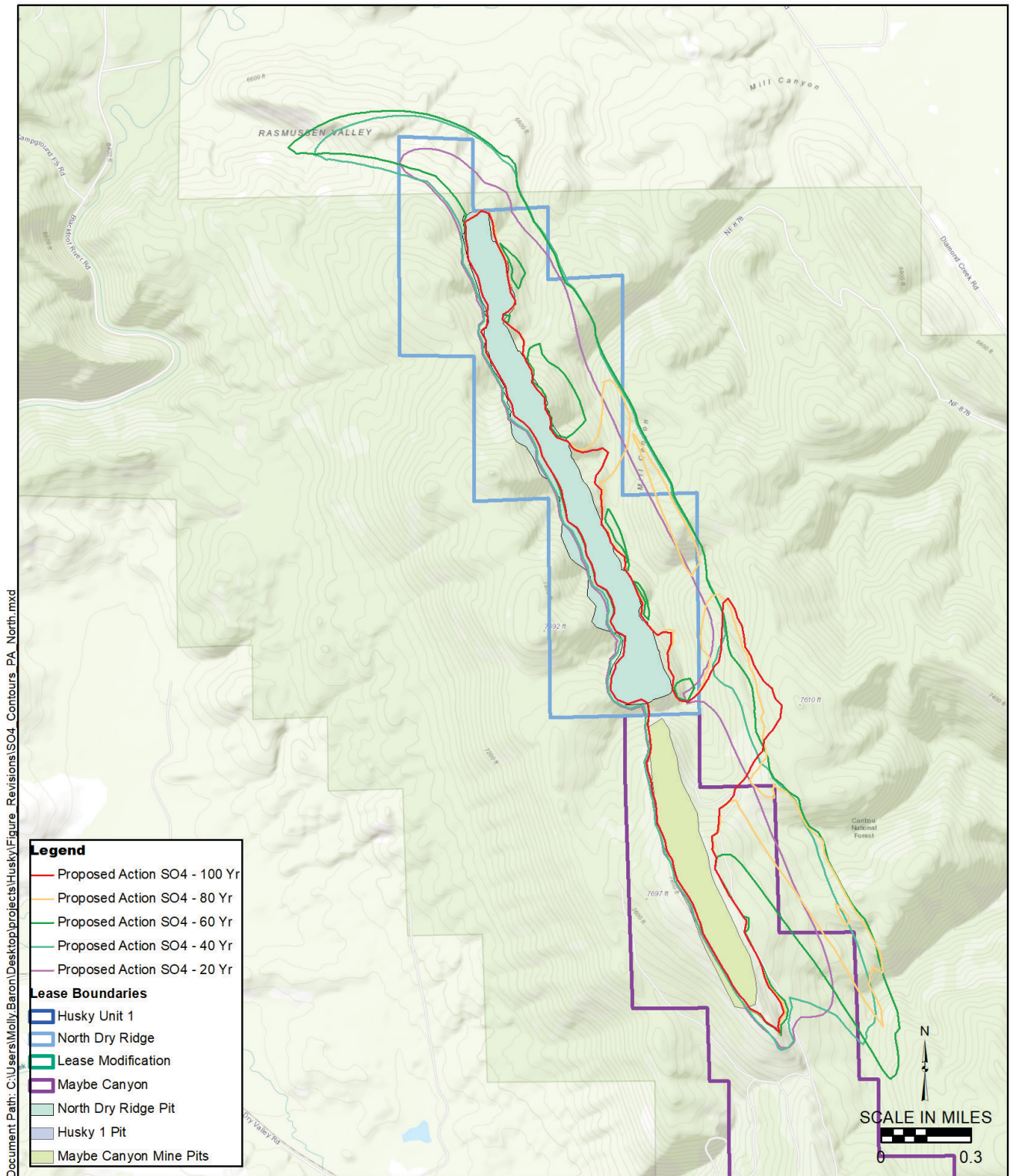
Figure 25. Proposed Action Predicted Extents of Sulfate Plumes at 20-Year Intervals from NDR and North Maybe Mine
