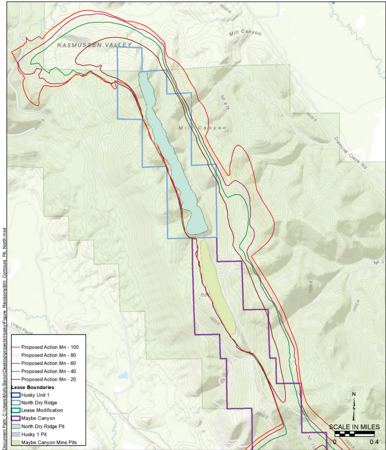
Figure 23. Proposed Action Predicted Extents of Manganese Plumes at 20-Year Intervals from NDR and North Maybe Mine
