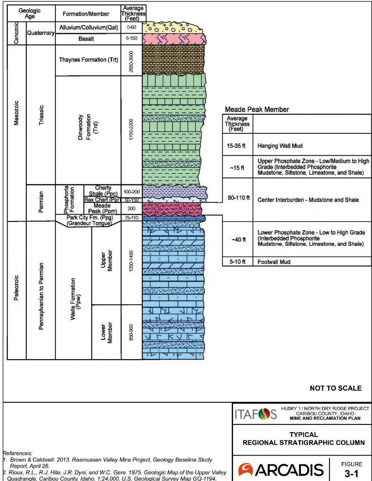
Figure 17. Regional Stratigraphic Column
