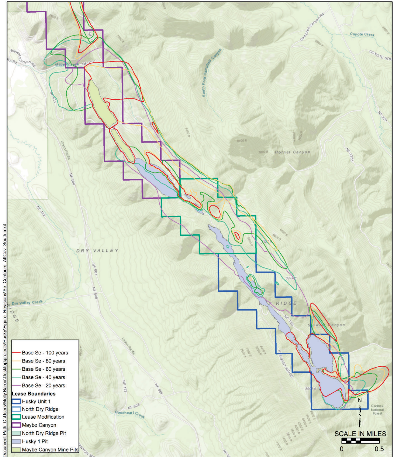
Figure 28. Alternative Cover Extent of Selenium Contamination at 20-Year Intervals from South Maybe Canyon Mine and H1
