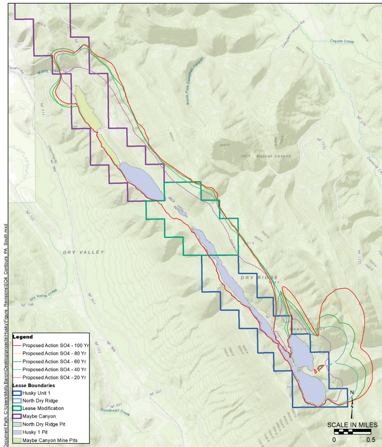
Figure 26. Proposed Action Predicted Extents of Sulfate Plumes at 20-Year Intervals from South Maybe Canyon Mine and H1
