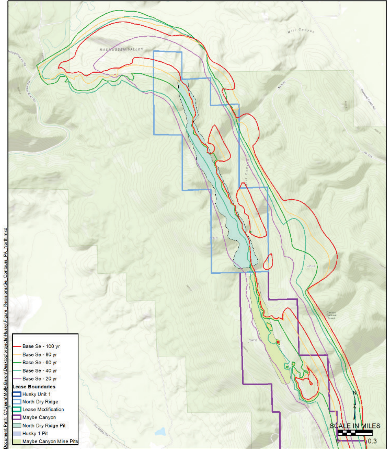
Figure 21. Proposed Action Predicted Extents of Selenium Plumes at 20-Year Intervals From NDR and North Maybe Mine
