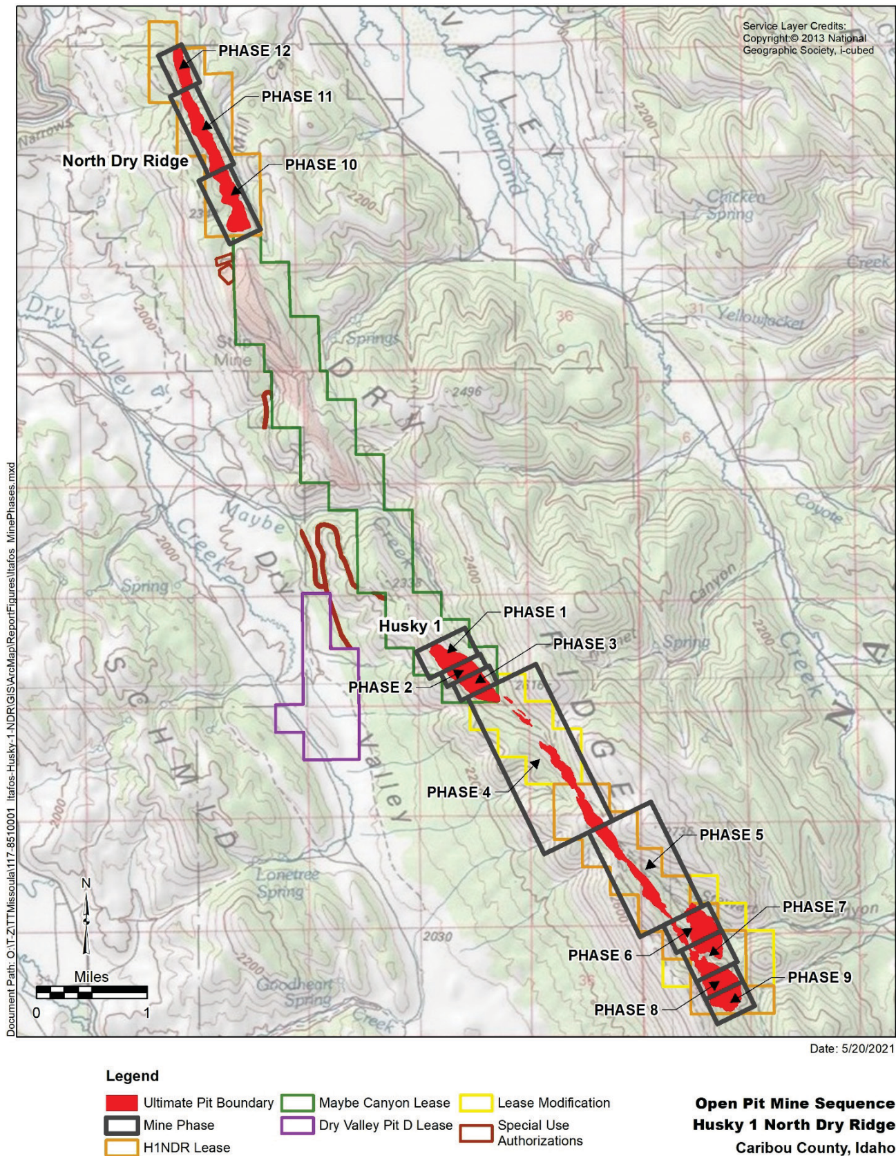
Figure 5. Open Pit Mine Sequence
